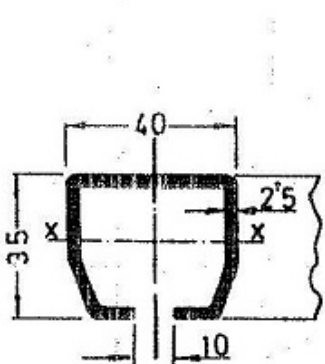
Perfil - Ref. 2.500-1
