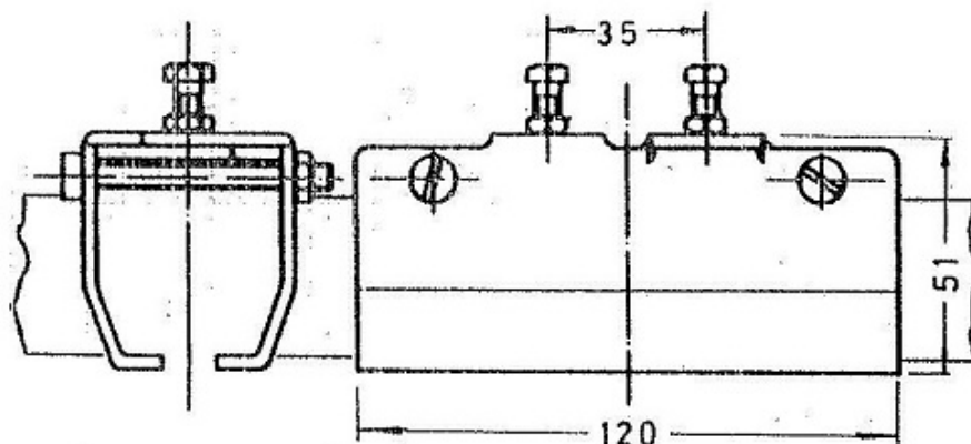
Empalme - Ref. 2.500-3
