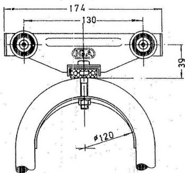
Intermedio - Ref. 2.500-5
