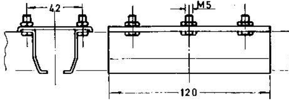
Empalme - Ref. 2.401-3
