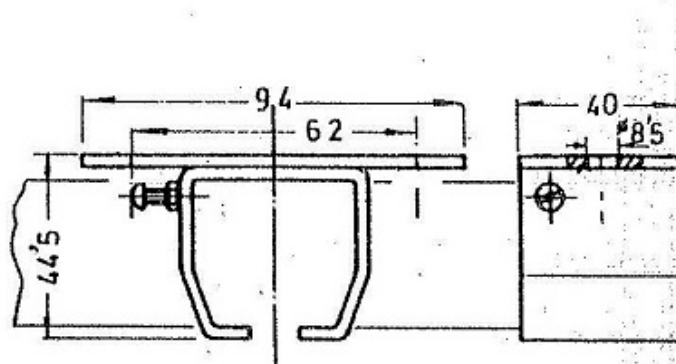
Soporte - Ref. 2.500-4
