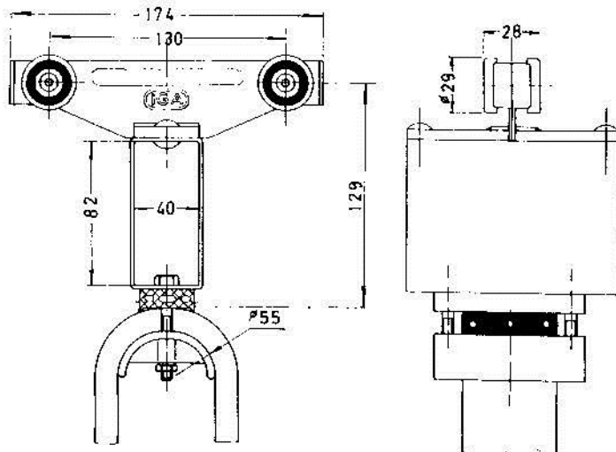
Arrastrador - Ref. 2.500-100-6
