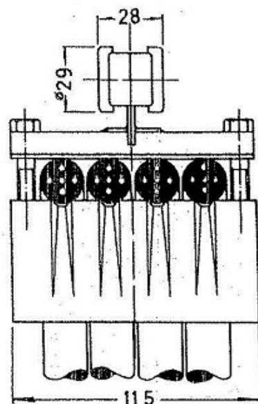
Intermedio - Ref. 2.500-5
