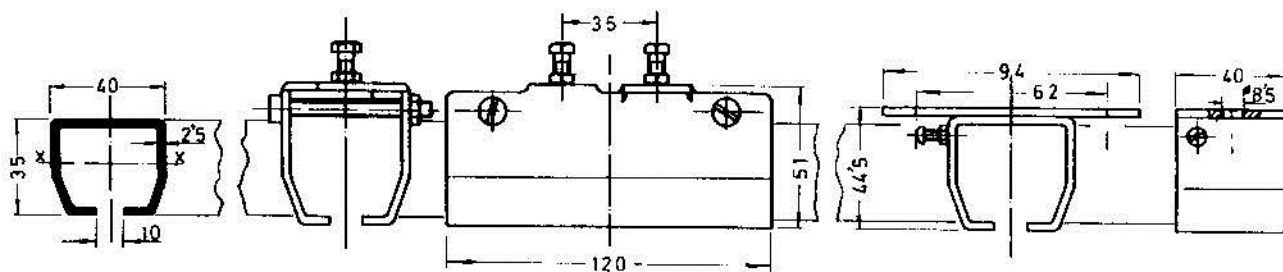
Perfil - Ref. 2.500-100-1
