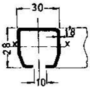
Perfil - Ref. 2.401-1
