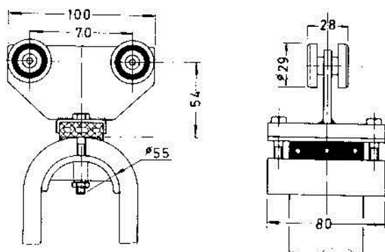
Intermedio - Ref. 2.500-100-5
